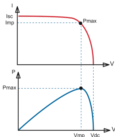
Zonne-laadcontroller MPPT 150/100-MC4
